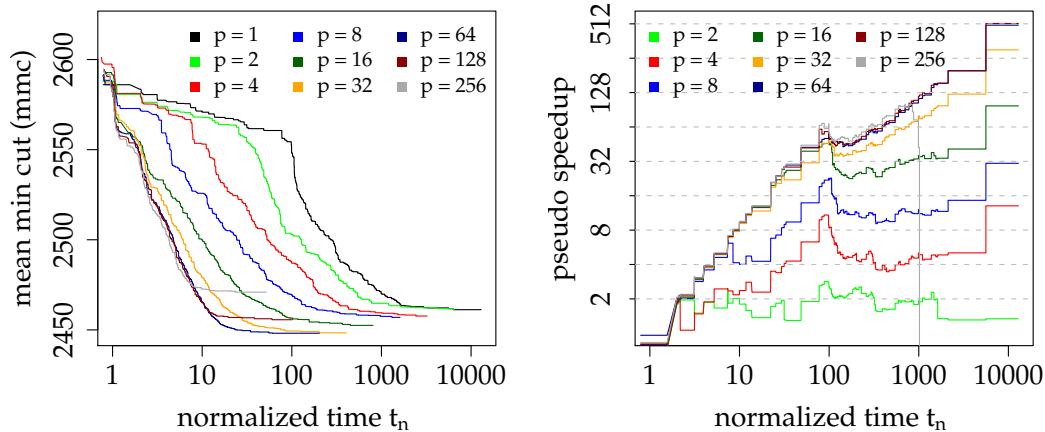
Figure 5.6: Scalability of our algorithm: (left) a normal convergence plot, (right) pseudo speedup S_p(t_n) . Source: [144].
