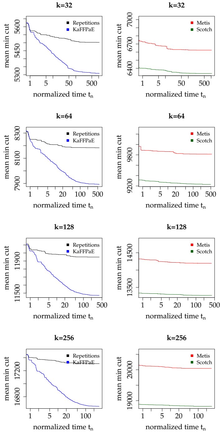
Figure 7.7: Convergence plots for the comparison of solution quality of KaFFPaE with repeated executions of KaFFPa, Scotch and Metis (over time) ( k \in \{32, \dots, 256\} , \varepsilon = 3\% ).
