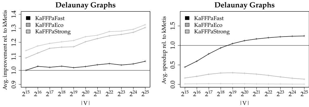
Figure 4.16: Results for Delaunay Graphs. Source: [143].
