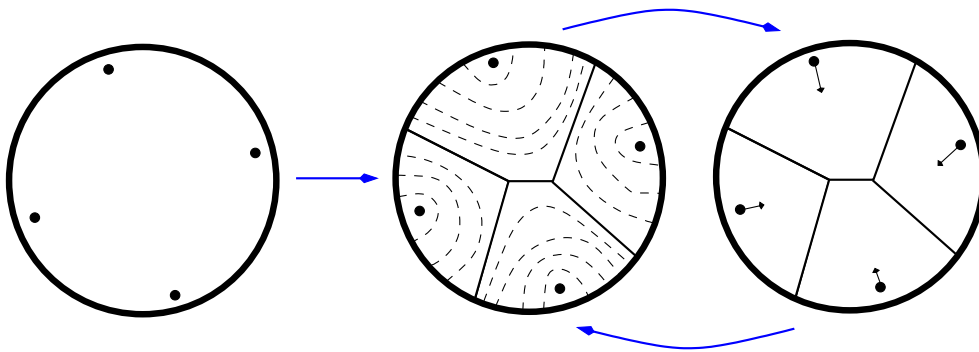
Figure 3.4: The three steps of the bubble framework. Black nodes indicate the seed nodes. On the left hand side, seed nodes are found. In the middle, a partition is found by performing breadth-first searches around the seed nodes and on the right hand side new seed nodes are found.
