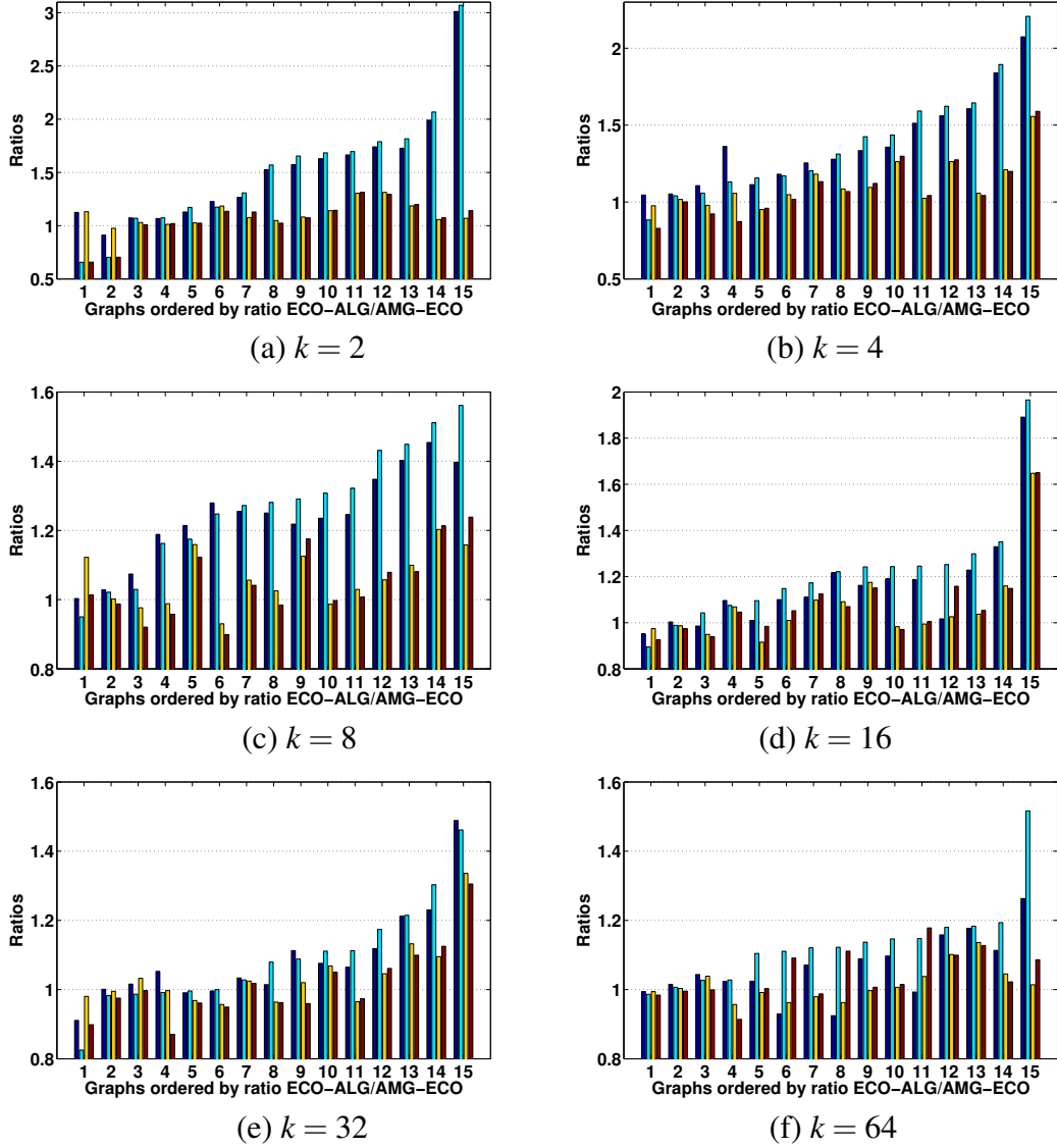
Figure A.3: Comparison of coarsening schemes on scale-free graphs. Figures (a)-(f) contain results of comparison for k = 2, 4, 8, 16, 32 , and 64 , respectively. Each quadruple of bars correspond to one graph. First, second, third and fourth bars represent averages of ratios ECO/AMG-ECO, ECO-ALG/AMG-ECO after local search, ECO/AMG-ECO, and ECO-ALG/AMG-ECO before local search, respectively.
