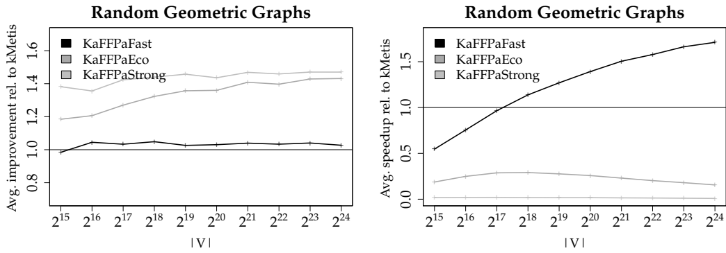
Figure 4.15: Results for Random Geometric Graphs. Source: [143].
