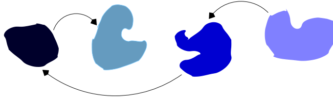
Figure 5.4: Islands of the evolutionary algorithm. Each PE has its own population and performs combine and mutation operations using different random seeds. From time to time the locally best partition is send to other PEs. Source: [144].
