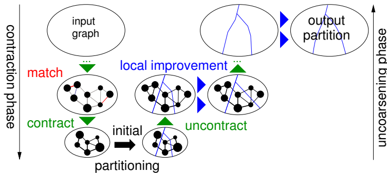
Figure 3.5: The multilevel approach to graph partitioning. Source: [143] 2 .
