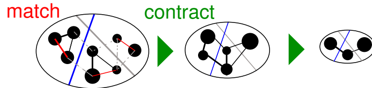
Figure 5.1: A graph G with two partitions, the dark and the light line, are shown. Cut edges are not eligible for the matching algorithm. Contraction is done until no matchable edge is left. The best of the two given partitions is used as initial partition. Source: [144].
