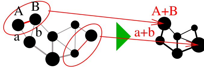
Figure 3.6: A example matching highlighted in red and contraction of matched edges. Source: [123].
